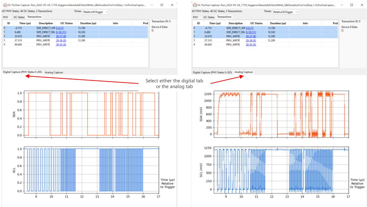
PurVue Analyzer™ Captures Showing Exact Time Correlation Between Digital and Analog Waveforms
