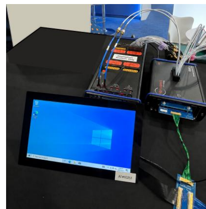
Probing an Embedded DisplayPort Application with the SV7C-eDP Analyzer and RSH2 Remote Sampling Head
